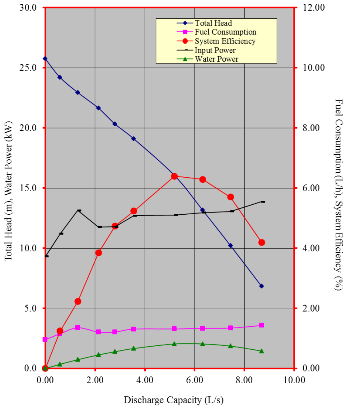
Figure 2. Performance characteristic curves of the ROBIN PTG207 self-priming centrifugal pumpset
